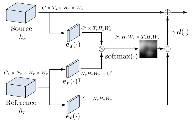
Fig. 5. Overview of the source-reference attention layer. This layer takes both a set of reference feature maps h_r and a set of source feature maps h_s as an input, and outputs a new set of feature maps of the same dimension as the source feature maps. This attention allows using non-local features from the reference features to perform a transformation of the source reference features. This transformation is done while conserving the local information similar to a purely convolutional layer. We denote matrix multiplication as “ \otimes ” and matrix addition as “ \oplus ”. The input and output dimensions of the different components are shown for reference.
