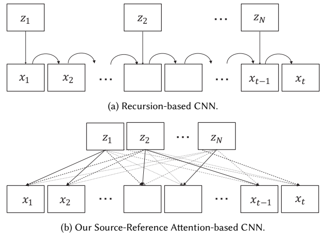
Fig. 3. Comparison between recursion-based and attention-based Convolutional Neural Networks (CNN) when processing an input video x with reference images z . Recursion-based networks simply propagate the information frame-by-frame, and because of this can not be processed in parallel and are unable to form long-term dependencies. Each time a new reference image is used, the propagation is restarted, and temporal coherency is lost. Source-reference attention-based networks, such as our approach, are able to use all the reference information when processing any the frames.
