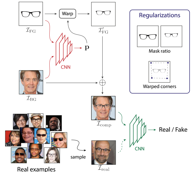
Figure 1. Overview of our image compositing pipeline. Given a foreground and background image, our single-shot placement model produces plausible image warping parameters to place the foreground image on the background. We propose a simple yet effective regularization to stabilize the adversarial training of the spatial transformer network.
