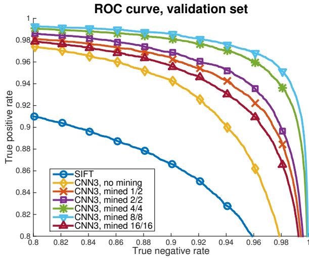
Figure 8: ROC curves for the experiments of Sec. 4.1.
