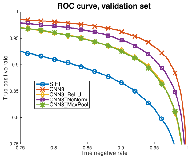
Figure 5: ROC curves for the experiments on hidden units, normalization, pooling.
